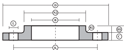
Slip-on Boss Flange
