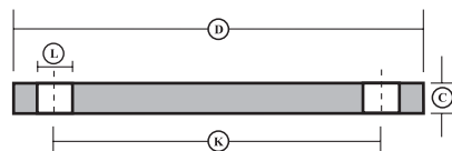
Steel Plate Blind Flange
