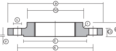
Screwed Boss Flange Up to 100 only
