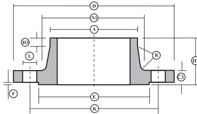
Steel Welding Neck Flange
